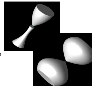
Two examples of bicones with non-linear sides
