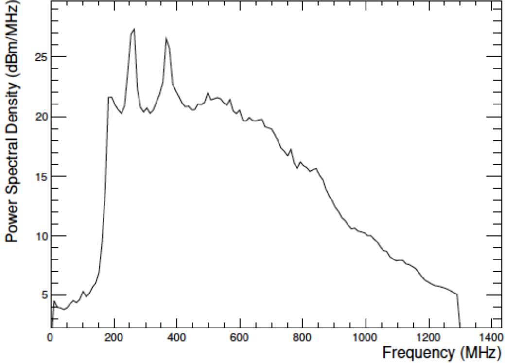
Figure 10: A plot of the average power spectral density over 1 min for one channel from when the ANITA-III payload was near WAIS Divide in Antarctica. The two peaks at 260 MHz and 375 MHz, presumably from military satellites, are visible here. The 260 MHz peak was present throughout the flight and the 375 MHz peak was present during less than half of the flight. These CW peaks motivated the installation of the TUFF notch filters in ANITA-IV. As it turns out, Notch 1 (to curb the left peak) and Notch 2 (to curb the right peak) both needed to be active for essentially the entire flight in ANITA-IV.
